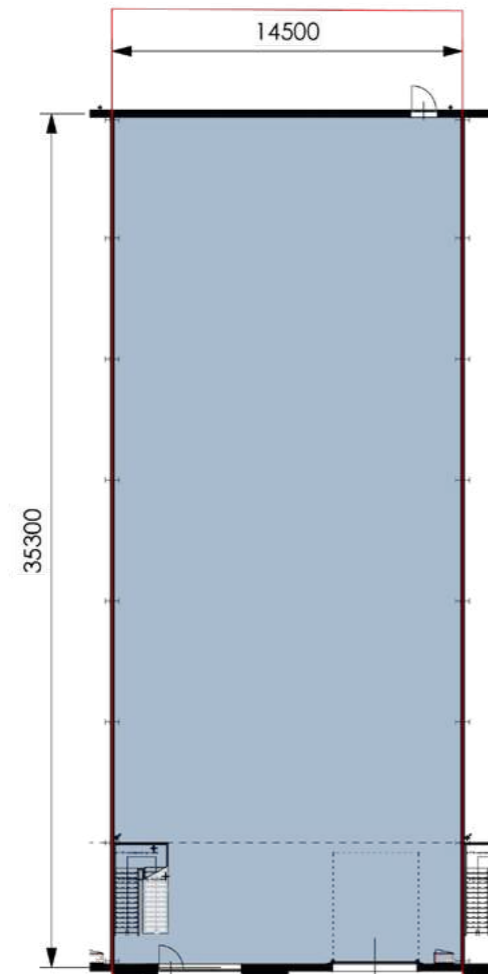
Begane grond - Unit 3 GO ±502 m 2
