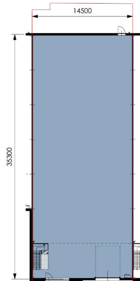
Begane grond - Unit 5 GO ±502 m 2
